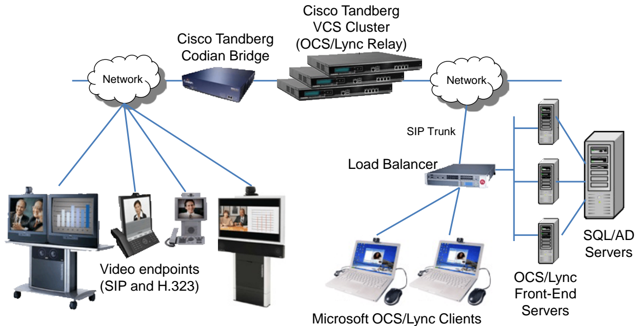
Figure 2. A global video network using Cisco Tandberg VCS clusters and Codian bridges. VCS clusters and Codian bridges are located in each regional video data center.
